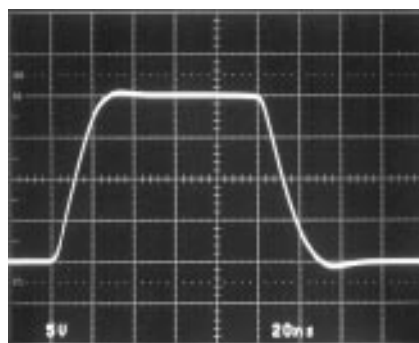
A_V = 10 R_F = 560\Omega R_G = 62\Omega V_S = \pm 15\text{V} R_L = 100\Omega
