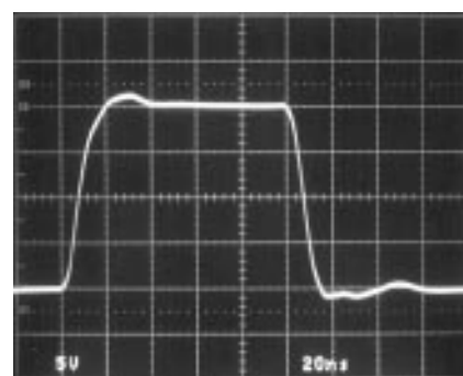
A_V = -1 R_F = R_G = 560\Omega V_S = \pm 15\text{V} R_L = 100\Omega
