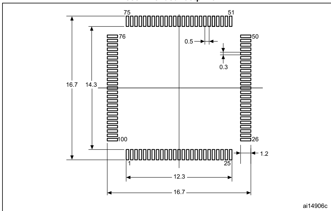
Figure 60. LQFP100 - 100-pin, 14 x 14 mm low-profile quad flat package recommended footprint
