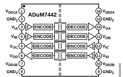
Figure 3. ADuM7442
