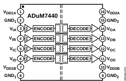
Figure 1. ADuM7440
