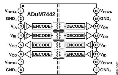
Figure 3. ADuM7442
