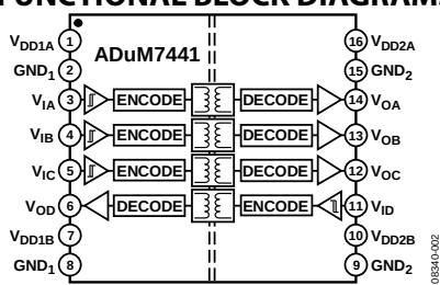
Figure 2. ADuM7441
