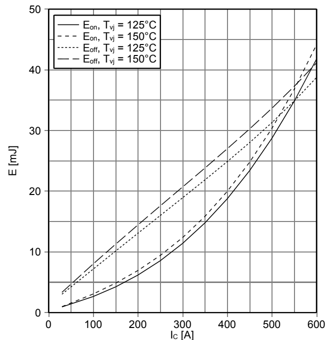
开关损耗 IGBT, T1 / T4 (典型) switching losses IGBT, T1 / T4 (typical)
