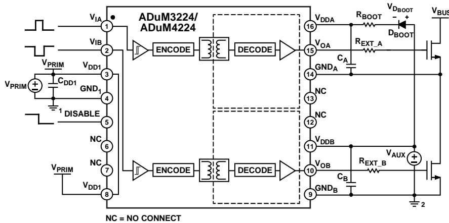
1 GND 1 IS CONNECTED TO THE PRIMARY SIDE GROUND, ISOLATED FROM THE SECONDARY GROUND. 2 GND B IS CONNECTED TO THE SECONDARY SIDE GROUND, ISOLATED FROM THE PRIMARY GROUND.
