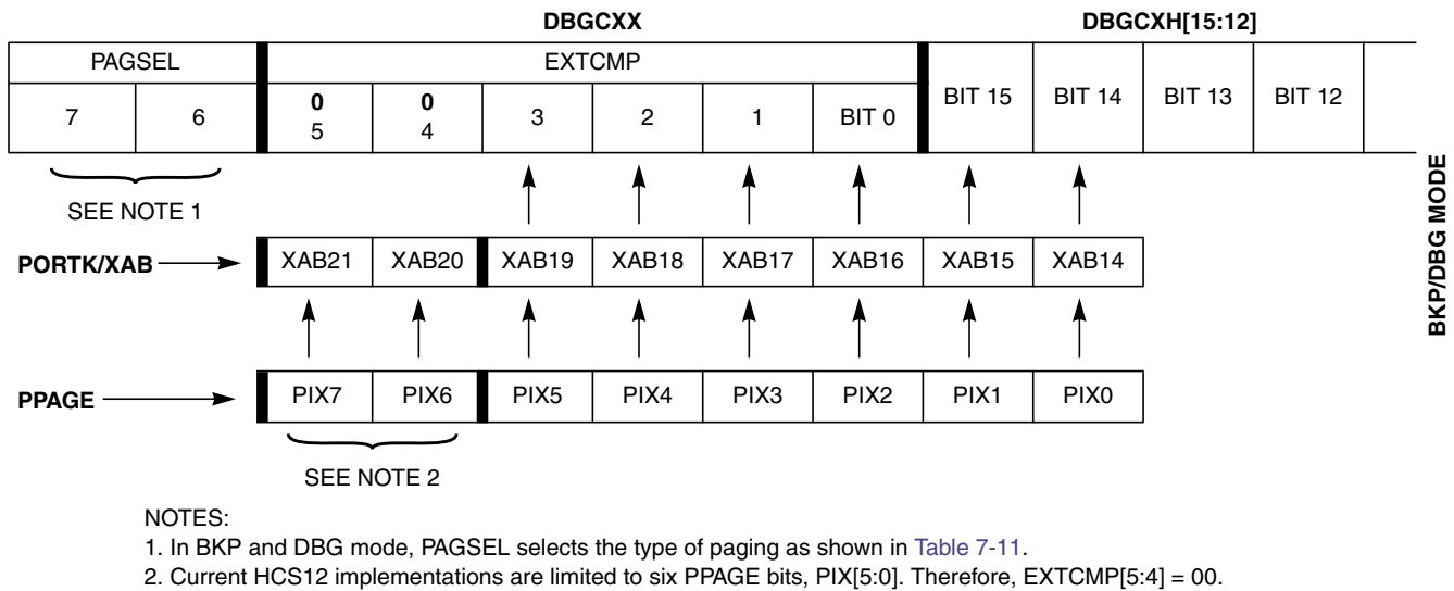
Figure 7-10. Comparator C Extended Comparison in BKP/DBG Mode
