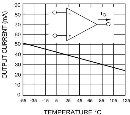
Figure 10: Current limiting
