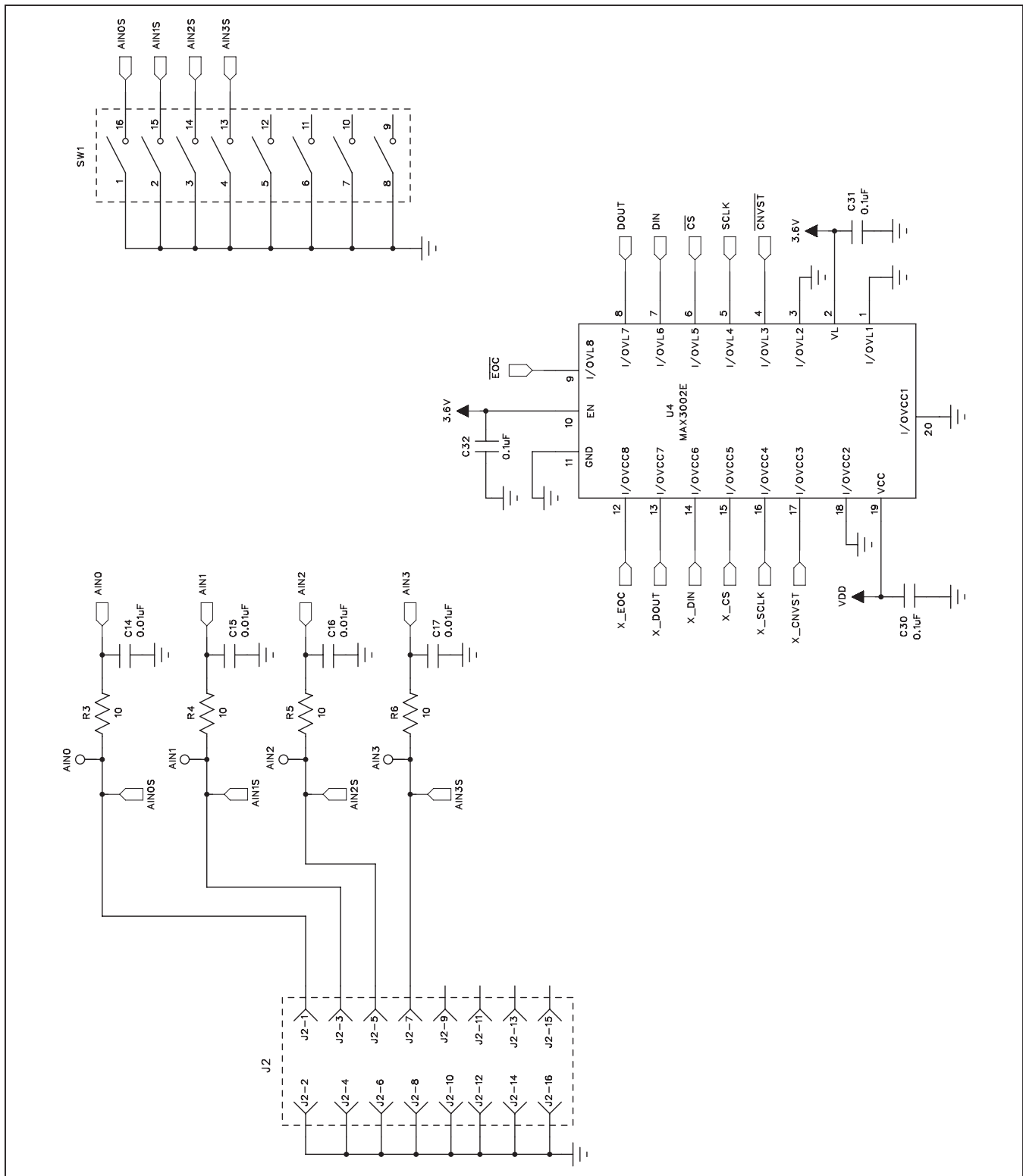
Figure 25b. MAX11635 Daughter Board Schematic (Sheet 2 of 2)
