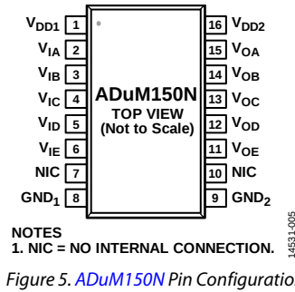
Figure 5. ADuM150N Pin Configuration
