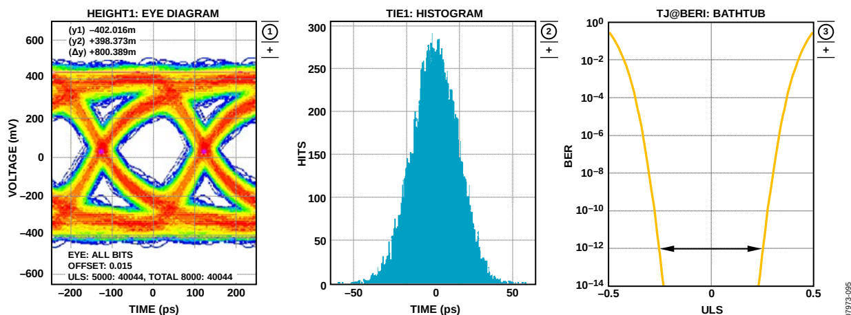
Figure 60. Digital Outputs Data Eye with Trace Lengths Greater Than 12 Inches on Standard FR-4, External 100 \Omega Terminations at Receiver
