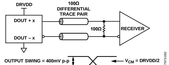
Figure 57. DC-Coupled Digital Output Termination Example
