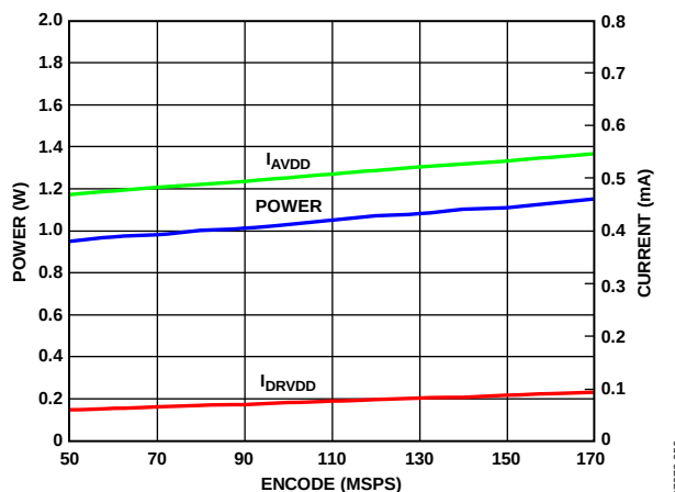
Figure 49. Supply Current vs. Encode for f_{IN} = 84.3 MHz, f_{SAMPLE} = 170 MSPS
