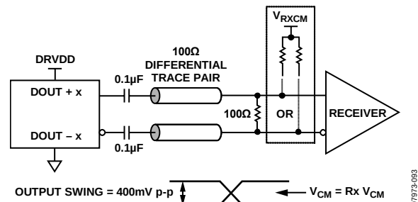
Figure 58. AC-Coupled Digital Output Termination Example
