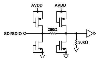
Figure 30. Equivalent SDI/SDIO Input Circuit
