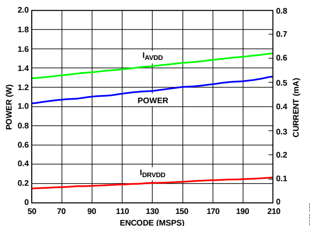
Figure 50. Supply Current vs. Encode for f_{IN} = 84.3 MHz, f_{SAMPLE} = 210 MSPS
