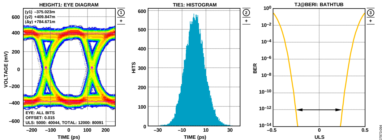
Figure 59. Digital Outputs Data Eye with Trace Lengths Less Than 6 Inches on Standard FR-4, External 100 \Omega Terminations at Receiver
