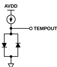
Figure 31. Equivalent TEMPOUT Output Circuit
