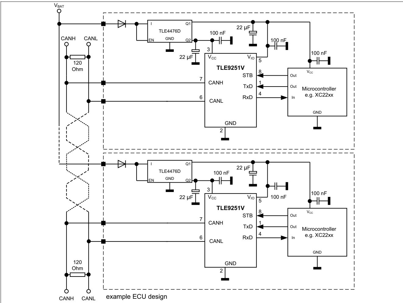
Figure 18 Application circuit
