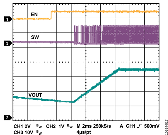
Figure 13. Soft Start with Precharged Output, 3.3 V_{OUT} Forced PWM
