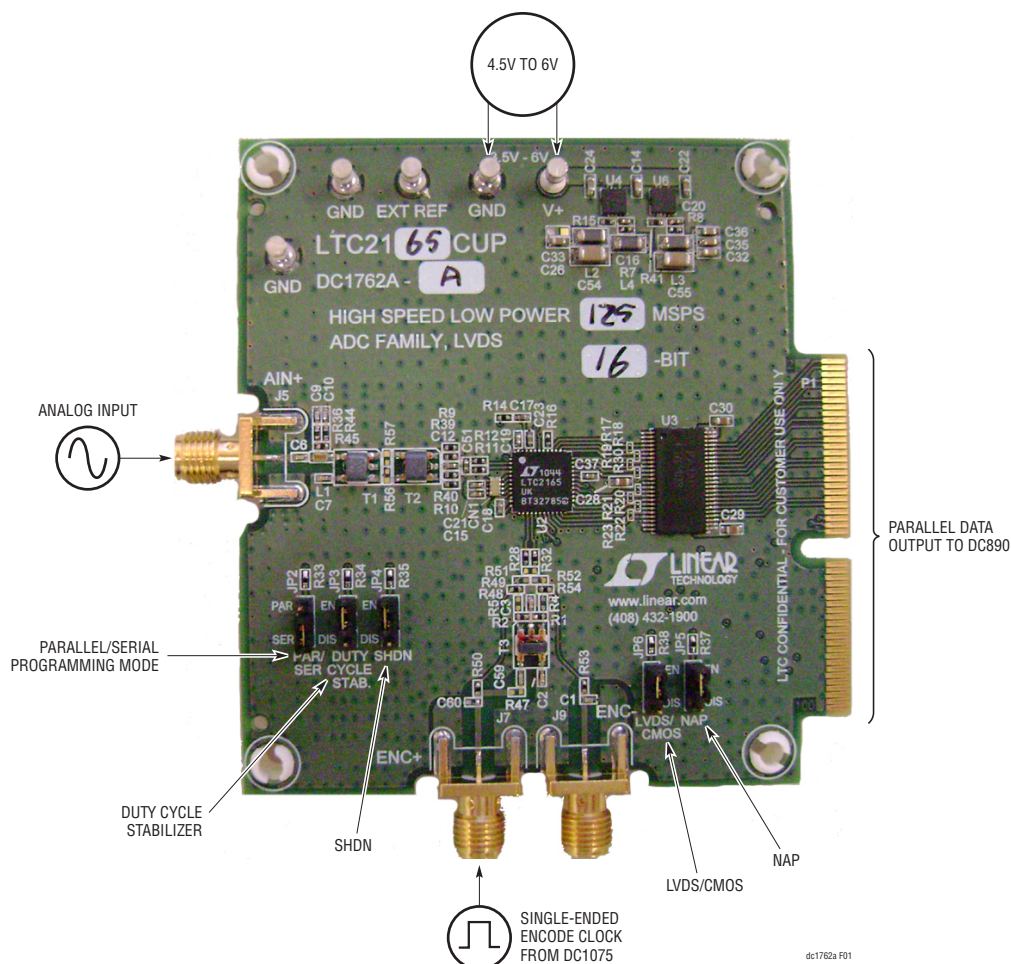
Figure 1. DC1762 Setup
