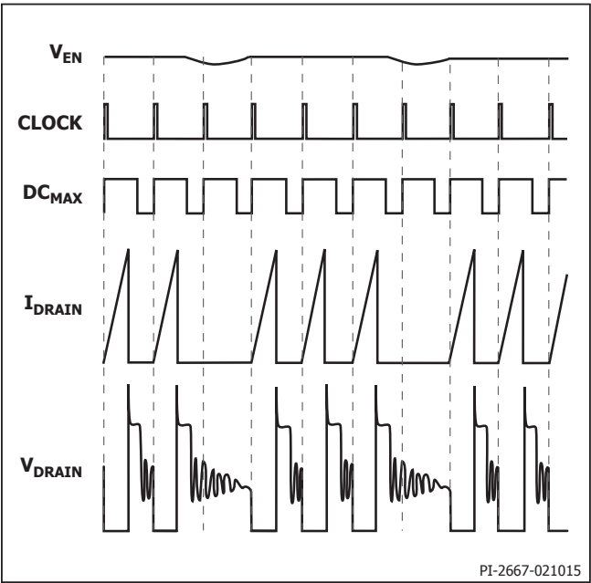
Figure 8. Operation at Moderately Heavy Loading.
