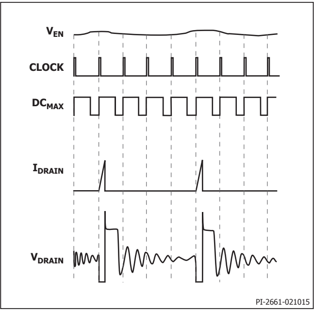
Figure 10. Operation at Very Light Load.
