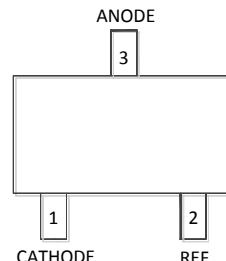
SOT23 (Package Code: N1)
