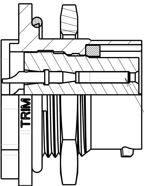
FEMALE CONNECTOR
