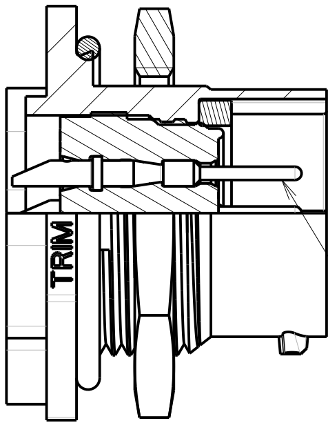
MALE CONNECTOR
