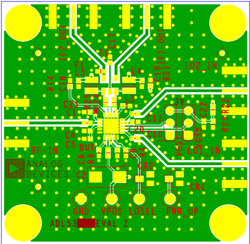
Figure 50. Evaluation Board Top Layer
