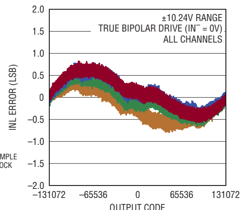
Integral Nonlinearity vs Output Code and Channel
