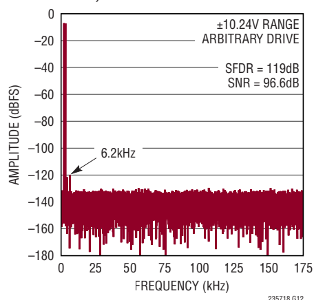
32k Point Arbitrary Two-Tone FFT f_{SAMPL} = 350\text{ksps} , IN^+ = -7\text{dBFS } 2\text{kHz} Sine, IN^- = -7\text{dBFS } 3.1\text{kHz} Sine
