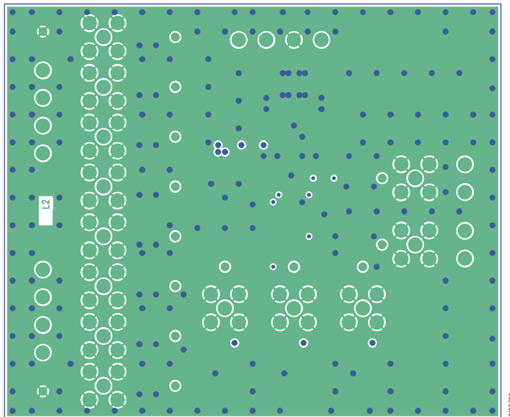
Figure 8. EVAL-ADG5209FEBZ Layer 2
