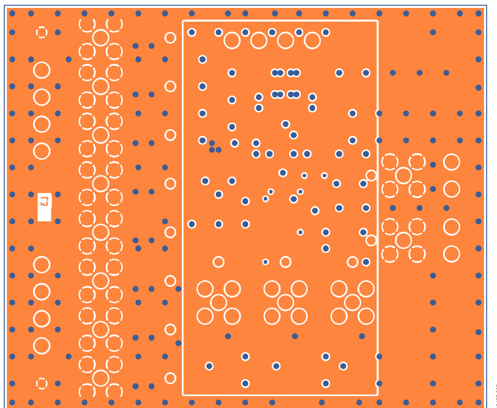
Figure 9. EVAL-ADG5209FEBZ Layer 3
