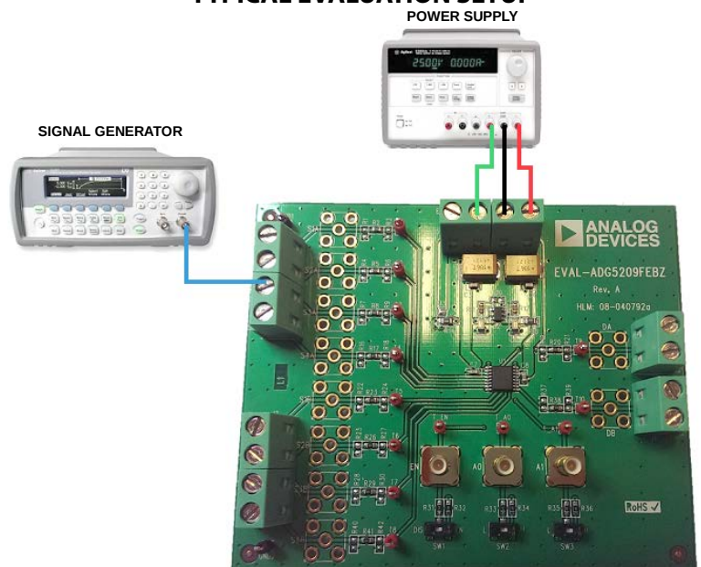
Figure 1. EVAL-ADG5209FEBZ , Power Supply, and Signal Generator
