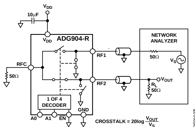
Figure 23. Crosstalk
