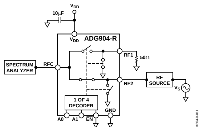
Figure 26. P-1 dB
