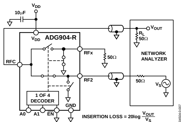
Figure 22. Insertion Loss
