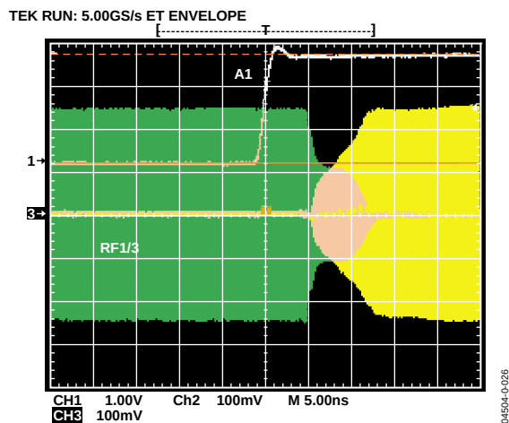
Figure 15. Switch Timing
