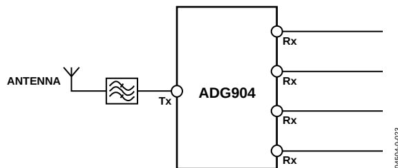
Figure 29. Tx/Rx Switching
