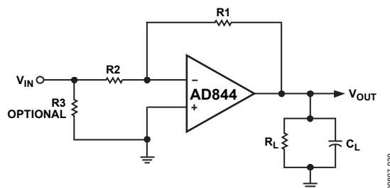
Figure 29. Inverting Amplifier
