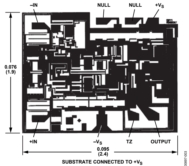
Figure 3. Die Photograph
