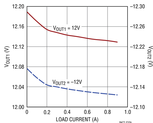
Figure 10c. 12V and -12V Outputs vs Load Current ( V_{CC} = 18V , Load from V_{OUT1} to V_{OUT2} )
