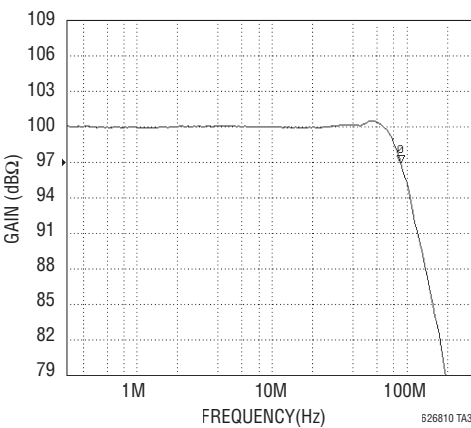
100kΩ TIA Frequency Response
