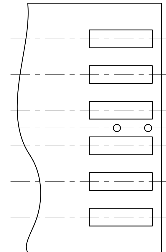
RECOMMENDED PCB LAYOUT FOR 2213504-3 & 1-2213504-3
