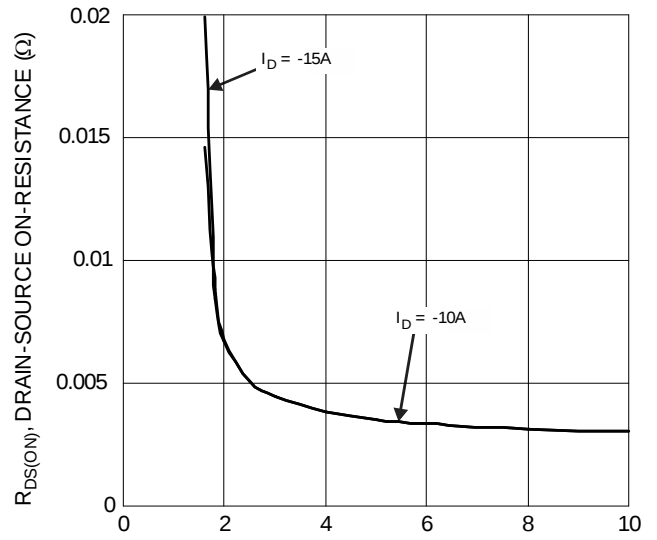
Figure 4 Typical Drain-Source On-Resistance vs. Gate-Source Voltage
