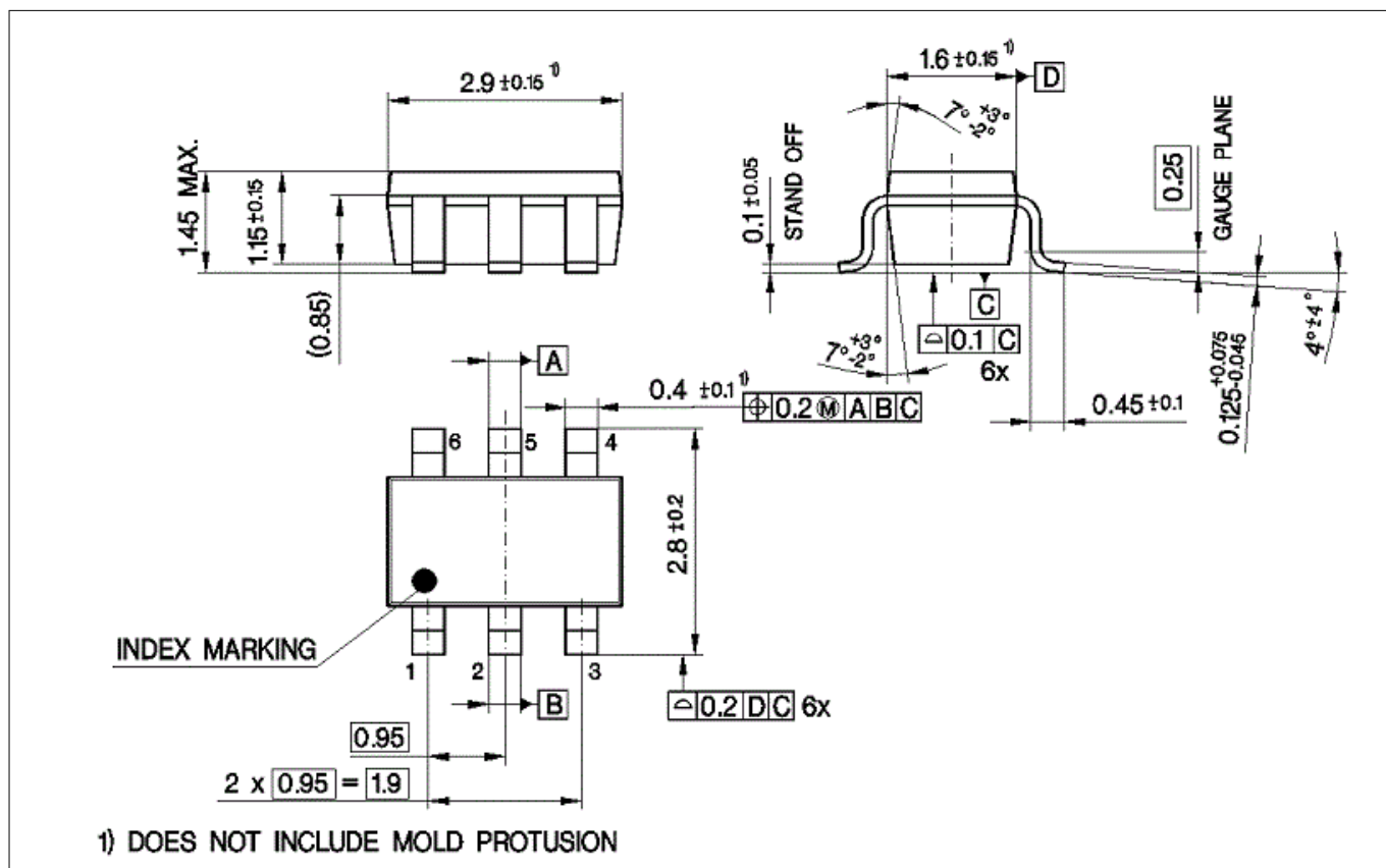
Figure 5 Package Drawings
