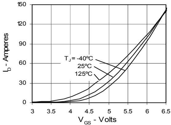
Fig. 7. Input Admittance
