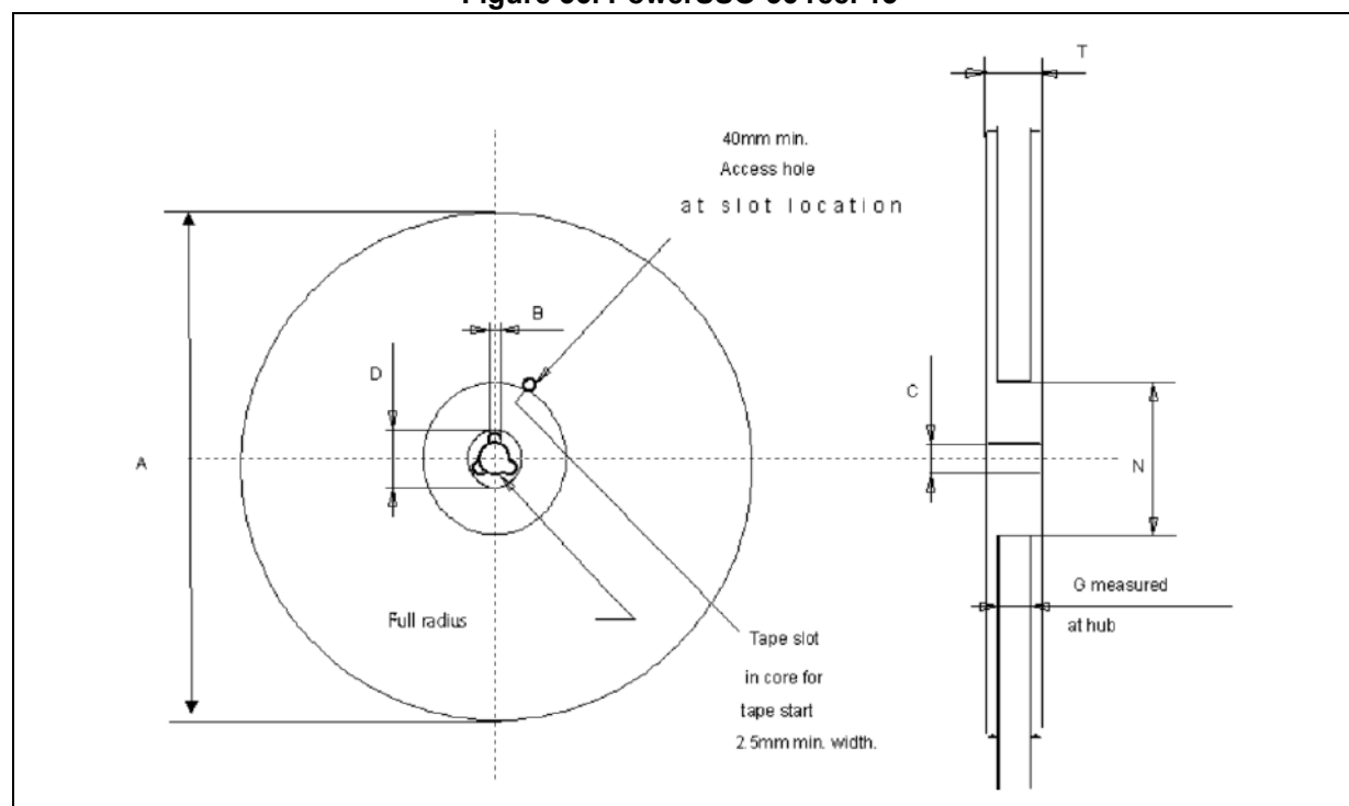
Figure 36. PowerSSO-36 reel 13"
