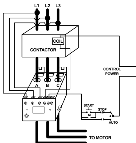
CURRENT TRANSFORMER WIRING DIAGRAM FOR 777-KW/HP-P2 SERIES
