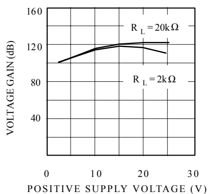
Figure 15. Voltage gain
