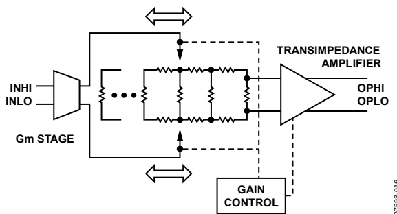
Figure 14. Simplified Schematic
