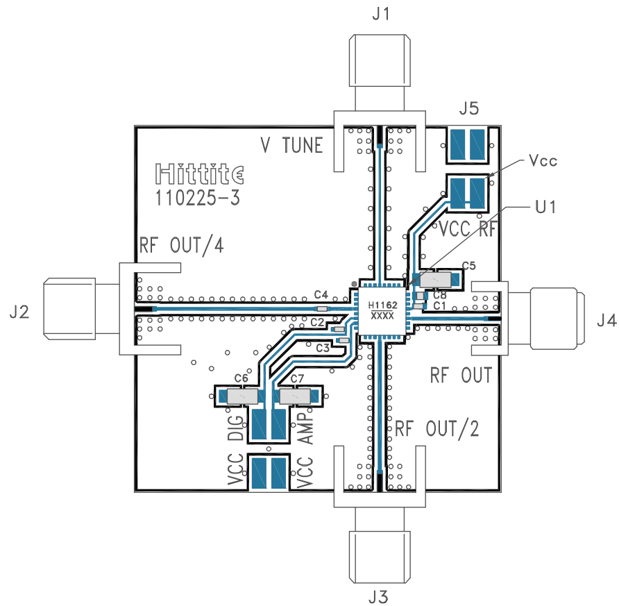
Figure 17. Evaluation Board
