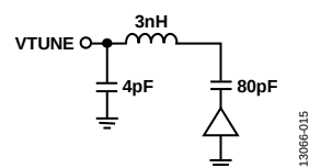
Figure 6. VTUNE Interface
