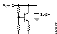
Figure 5. V CC Interface
