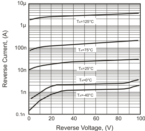
Fig.2 - Reverse Characteristics
