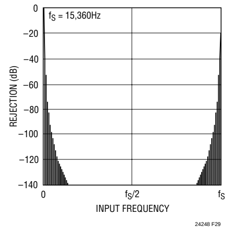
Rejection vs Frequency at V_{IN}
