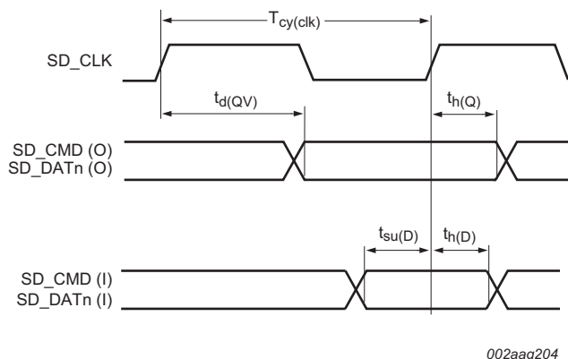
Fig 40. SD/MMC timing
