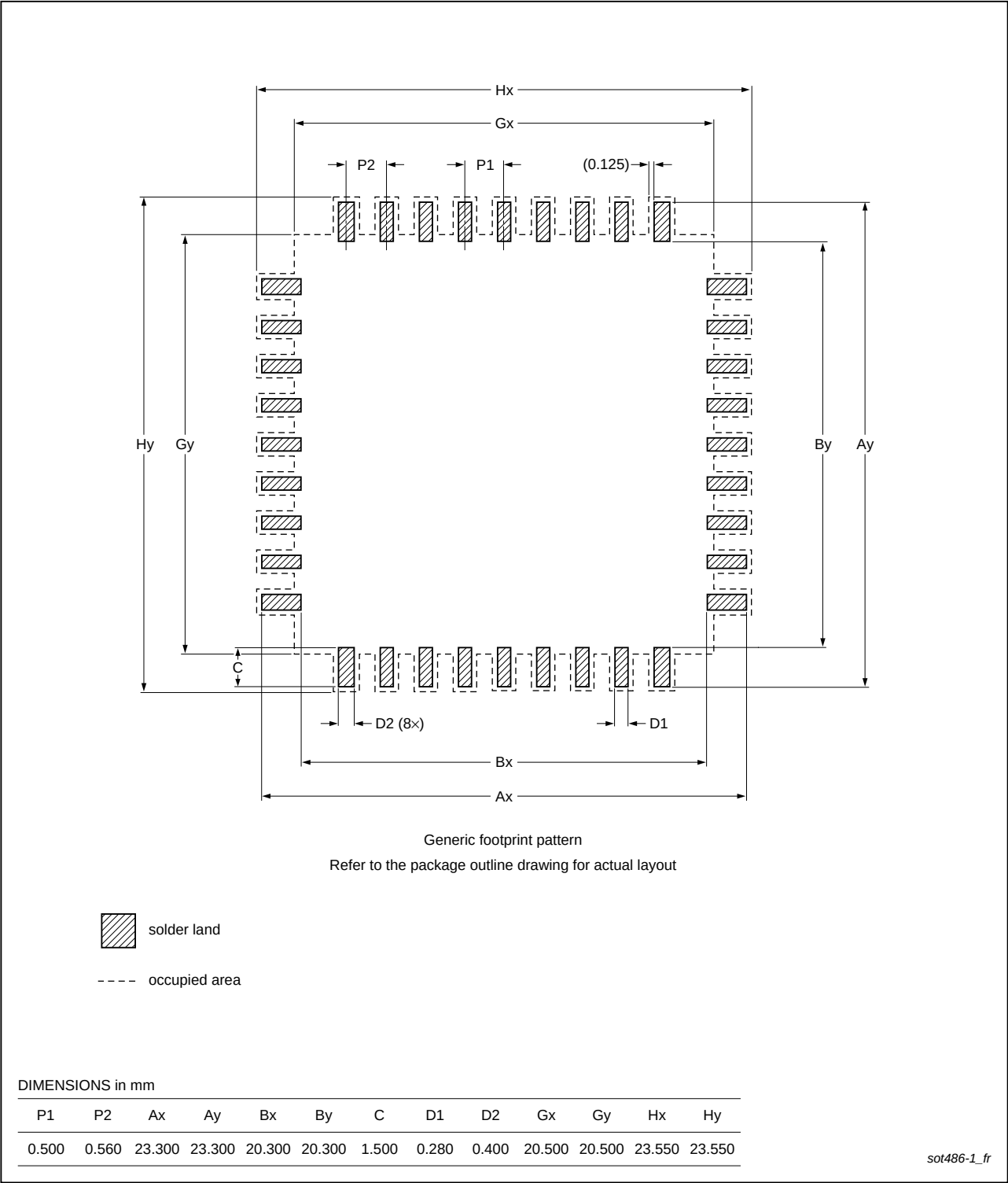
Fig 57. Reflow soldering of the LQFP144 package
