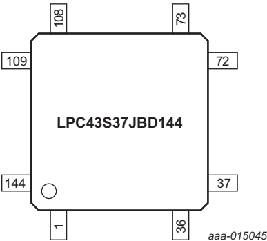
Fig 5. Pin configuration LQFP144 package
