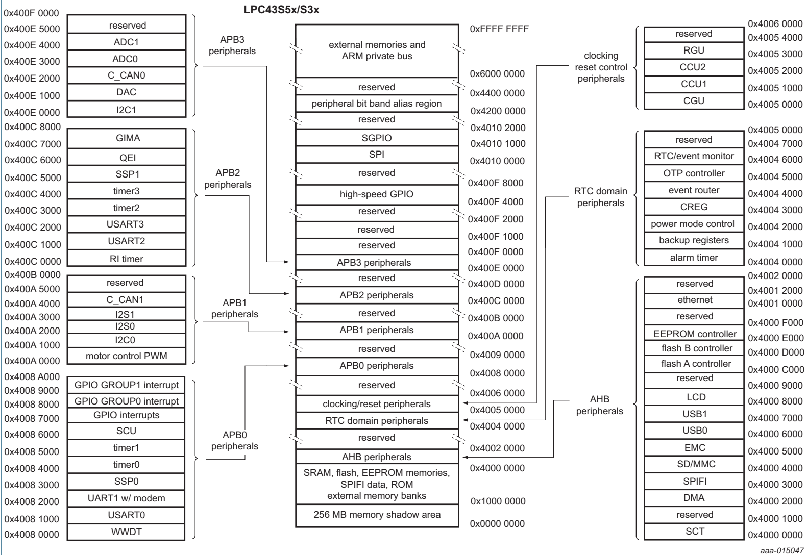
Fig 8. LPC4355x/S3x Memory mapping (peripherals)
