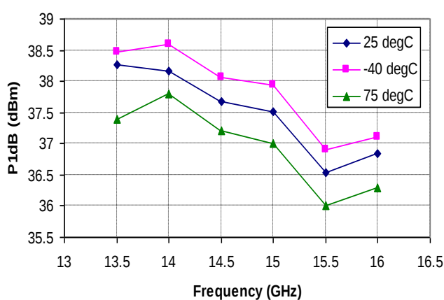
P1dB vs. Frequency vs. Temperature
