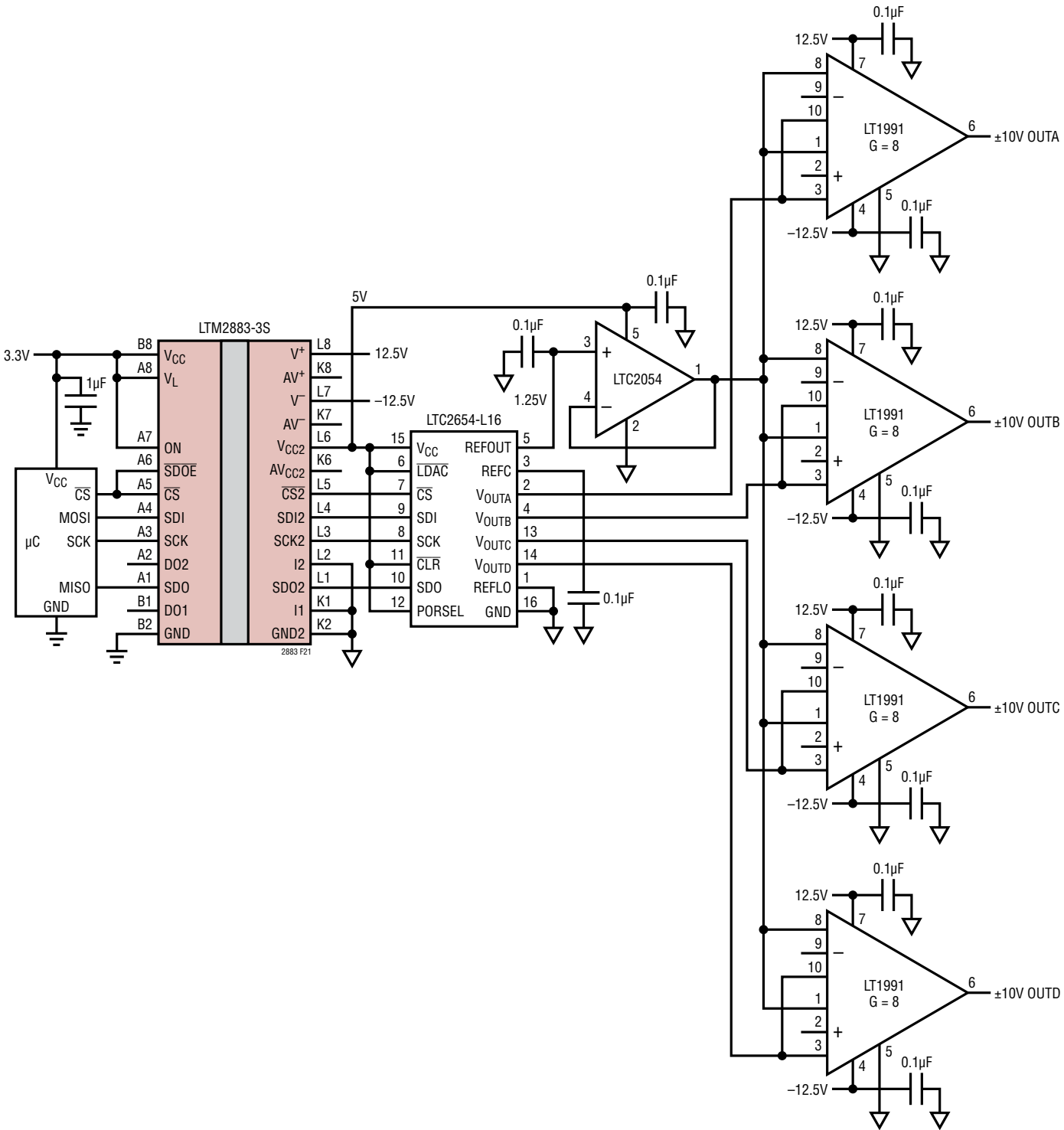
Figure 21. Quad 16-Bit \pm 10\text{V} Output Range DAC
