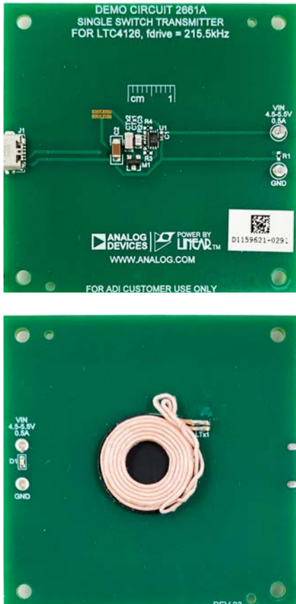
Figure 8. DC2661A Top/Bottom
