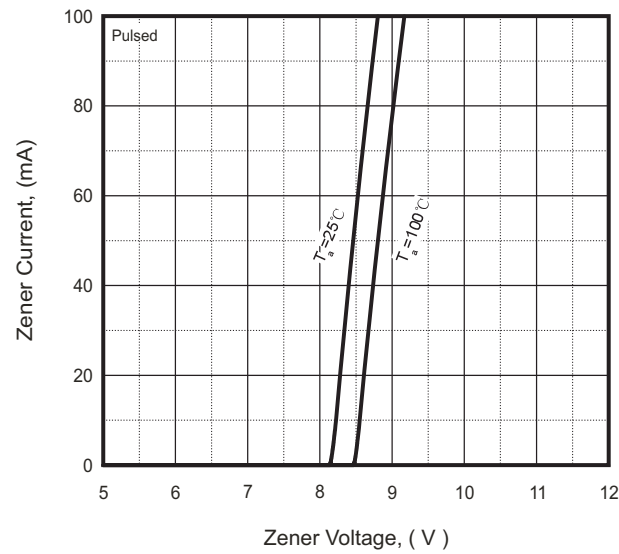
Fig.3 - Reverse Characteristics
