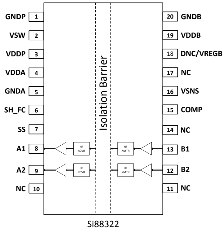
Figure 6.2. Si8832x Pinout Diagrams
