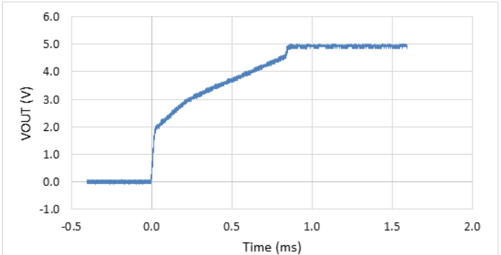
Figure 5.16. 24 V–5 V VOUT Startup vs. Time, No Load Current
