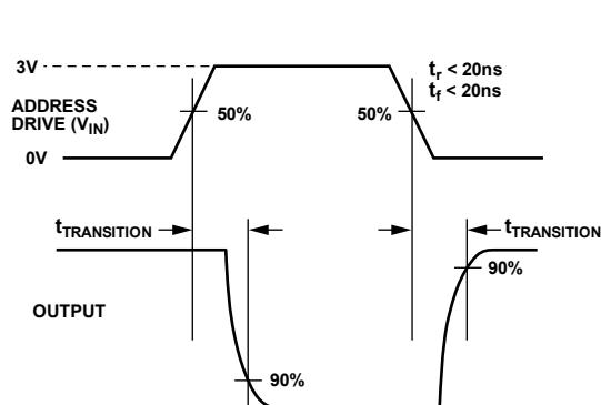
Figure 28. Address to Output Switching Times, t_{\text{TRANSITION}}
