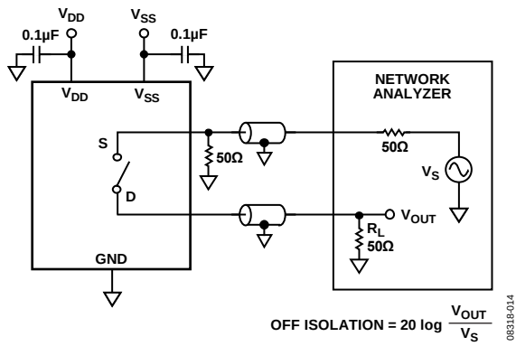
Figure 32. Off Isolation
