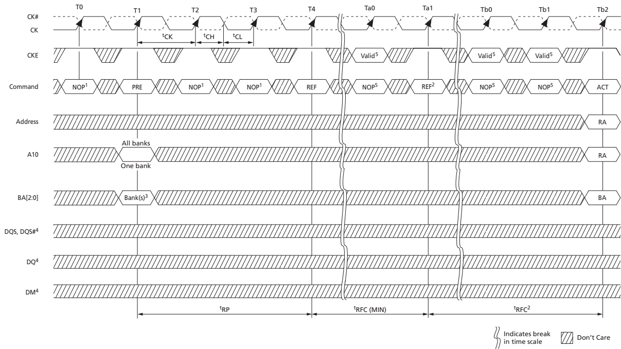
Figure 37: Refresh Mode
