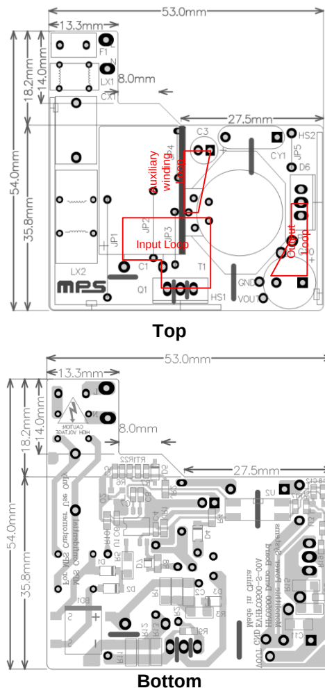
Figure 16: Recommended Layout
