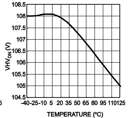
HV Turn-On Threshold vs. Temperature
