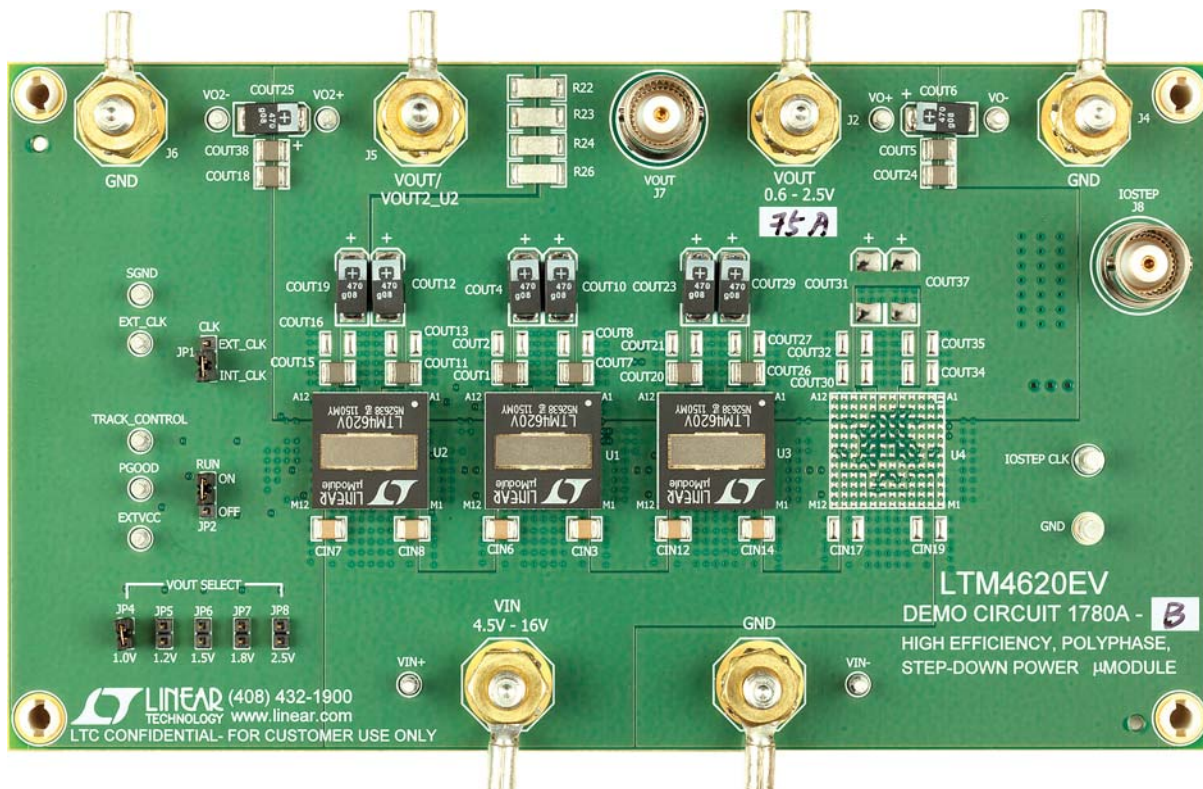
Figure 1. 75A PolyPhase LTM4620/DC1780A-B Demo Board
